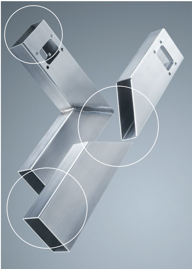
Conventionally welded from two single parts.
